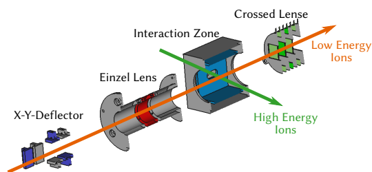
Figure 1. 3D model of the experimental area with indicated ion beams.
