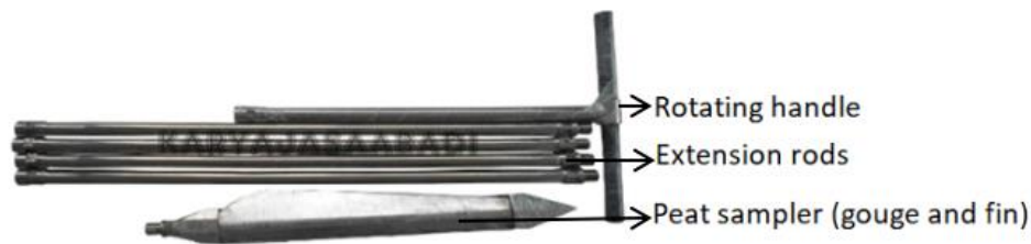
Figure 2. Peat auger Russian type
