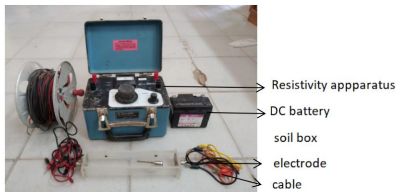
Figure 3. Soil resistance meter Nilsson S400
