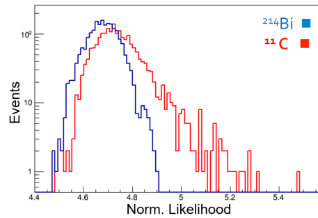
Figure 4: Reference PDFs of the \text{PS-}\mathcal{L}_{PR} pulse-shape discriminating variable for \beta^+ (red) and \beta^- events. ^{11}\text{C} events have in general higher values of the \text{PS-}\mathcal{L}_{PR} variable, which indicates a worse reconstructed position.
