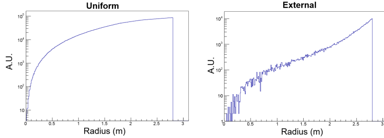
Figure 3: Reference PDFs for the radial distribution (integrated over energy) of uniformly distributed events ( Left ) and of external background events ( Right ) in the fiducial volume.
