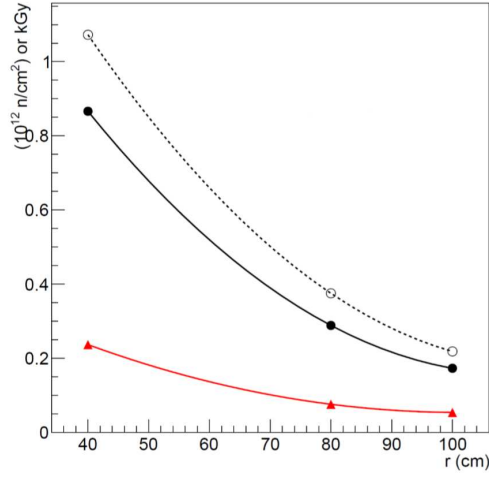
Figure 8. Ionizing (in kGy, \blacktriangle ) and non-ionizing (in \text{n}/\text{cm}^2 , \circ , and in \text{n-1MeV-eq}/\text{cm}^2 , \bullet ) doses as a function of the distance between the axis of the ENUBET decay tunnel and the inner radius of the calorimeter.
