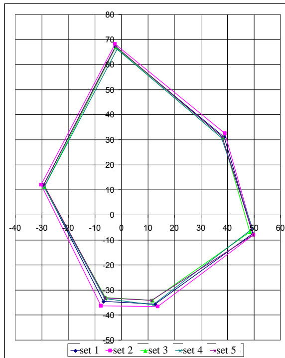
Figure 2. Hexagrams of color gamut of printing system No. 1 on the chromaticity diagram a^*b^* (the abscissa axis is a^* , the ordinate axis is b^* ; sets 1–5 of paper No. 1–5, respectively)
