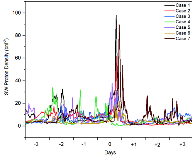
Fig. 2 Solar proton density variation during the same storm events investigated in this study. The super storm day is assigned 0 (zero), and + and – indicate the subsequent post- and pre- storm days respectively.
