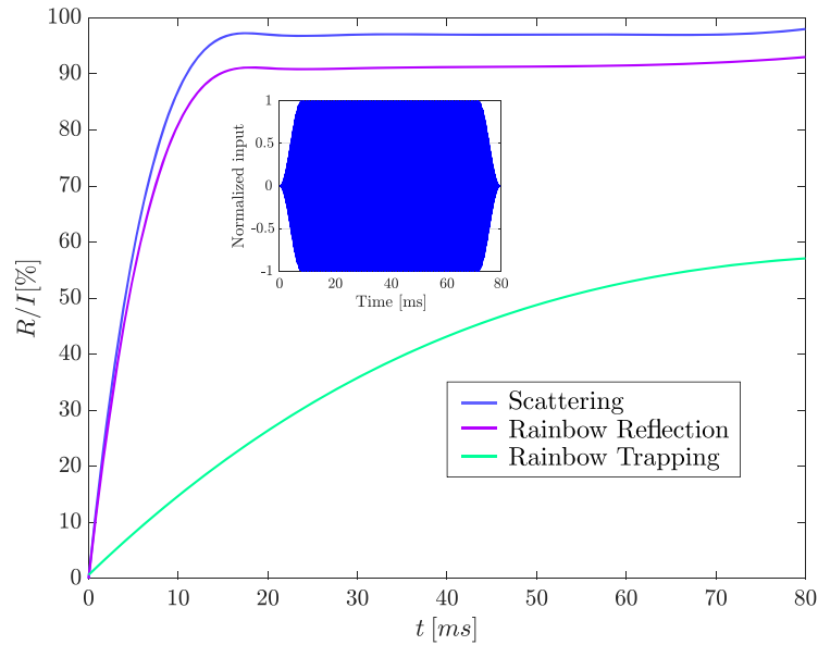
Figure 8. Percentage of reflected to input wave from polynomial interpolation for an 80 ms input (shown in inset), for the three arrays in figure 6. There is a clear reduction in reflection in the symmetry broken rainbow trapping array.
