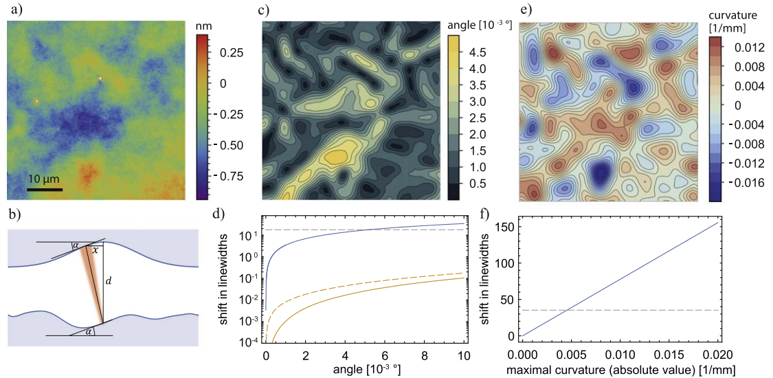
Figure 4. (a) White light interferometric measurement of the mirror surface. White spots are contaminants which are excluded from analysis. (b) Schematic illustration of the effect of local gradients of the planar mirror. (c) Calculated modulus of the local surface angle and (e) average curvature of the area shown in (a). (d) Change of \Delta\nu_{00,60} as a function of surface angle at q = 132 in units of \kappa . Yellow solid line: frequency shift due to changing r_c for an aligned cavity. Yellow dashed line: Shift due to changing r_c and changing penetration depth. Blue line: frequency shift due to r_c for an initial misalignment of \alpha_0 = 1.5^\circ . Gray dashed line: observed maximal shift. (f) Calculated change of transverse-mode frequency separation \Delta\nu_{00,60} as a function of the maximal local curvature in units of \kappa over the range of values observed in (a). Gray dashed line: Maximal shift observed in figure 3.
