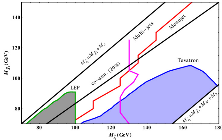
Figure 12. Tevatron and LHC limits on a light stop that decays to a charm quark and a neutralino LSP, \tilde{t}_1 \rightarrow c \tilde{\chi}_1^0 . Reprinted from He et al [184], copyright 2012 with permission from JHEP.
