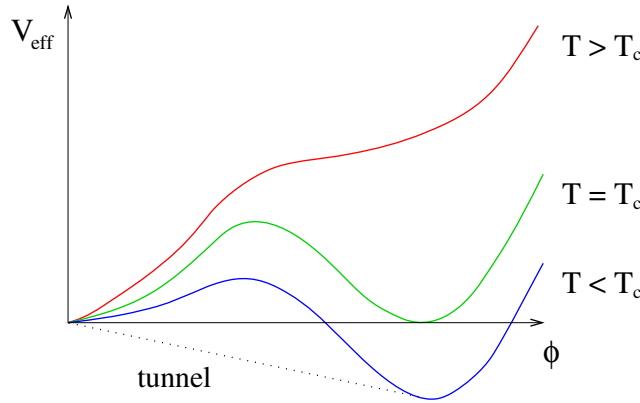
Figure 3. Schematic temperature dependence of the effective potential.
