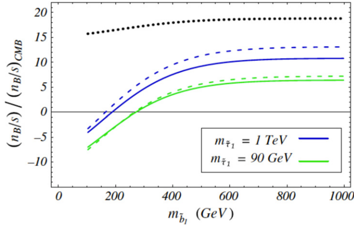
Figure 6. Baryon asymmetry as a function of RH bottom squark mass in the MSSM, scaled to the value obtained from the cosmic microwave background [113]. The blue (green) curves correspond to the RH tau mass of 1 TeV (90 GeV), while the black dotted line is obtained neglecting the bottom and tau Yukawa couplings. Solid curves give results of full numerical solution to transport equations, while the dashed line corresponds to an analytic approximation. A RH stop mass of 200 GeV has been assumed. Reprinted with permission from Chung et al [113], copyright 2009 by the American Physical Society.
