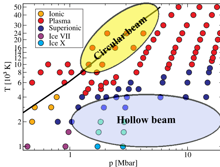
Figure 9. Each colored point corresponds to a QMD simulation in thermodynamic equilibrium. When the electronic conductivity exceeds 100 \text{ (ohm cm)}^{-1} [15], the ionic (dissociated) fluid is labeled as plasma. The solid line is the principal Hugoniot curve.
