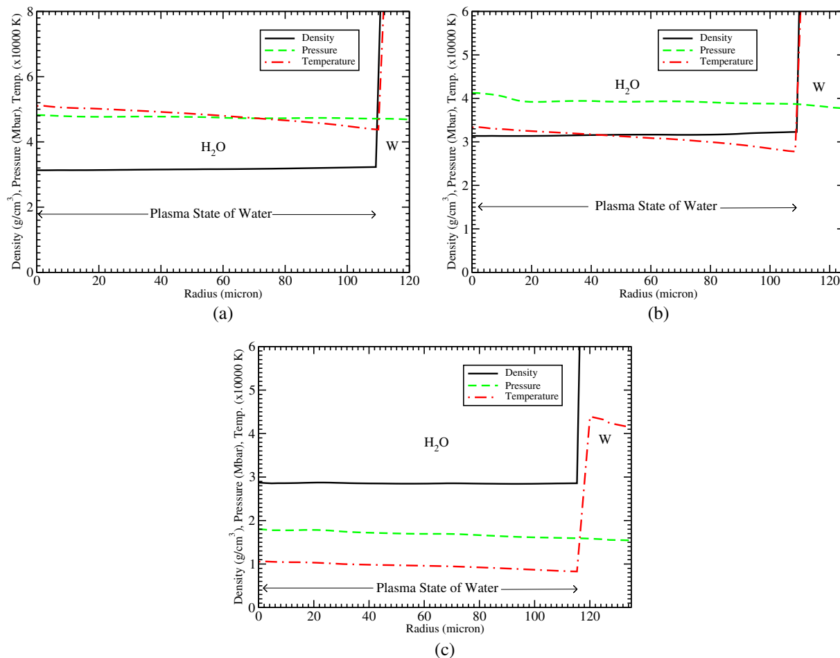
Figure 7. Density, temperature and pressure versus target radius at L = 3.5 mm in water at the time of maximum compression: (a) N = 5 \times 10^{11} , (b) N = 3 \times 10^{11} and (c) N = 10^{11} using a tungsten outer shell driven by a circular focal spot with FWHM = 1.5 mm.
