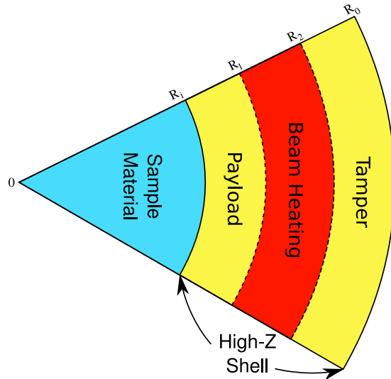
Figure 2. Cross-sectional view of the target shown in figure 1.
