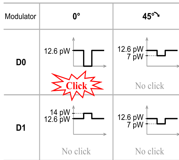
Figure 4. Proposed attack against a QKD system that uses two model 1 detectors: (a) equivalent optical scheme of Bob's setup; (b) scheme of the faked-state attack; (c) faked state sent by Eve in the case of her detection in the 0^\circ basis with the result D0, and the intensity diagrams that result at Bob's detectors for his two possible basis choices. Optical losses in components are neglected; in the presence of losses, Eve should send a proportionally brighter faked state.
