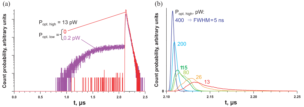
Figure 6. Detector model 1: time distributions of pulse's leading edge at the detector output, when Eve controls it by constant illumination with an approximately 2 \mu\text{s} wide gap: (a) time distributions for zero and nonzero P_{\text{opt, low}} (at P_{\text{opt, high}} = 13 \text{ pW} ); (b) time distributions in the main response peak for a range of P_{\text{opt, high}} values (at P_{\text{opt, low}} = 0 ). On the charts, t = 0 approximately corresponds to the start of the gap in illumination; the main response peak begins just after the end of the gap.
