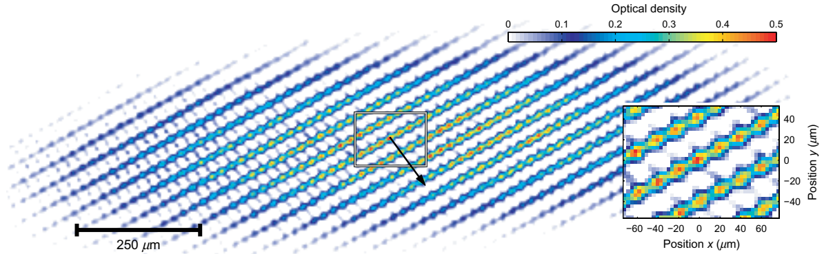
Figure 2. Loaded array of magnetic microtraps. An absorption image of the two-dimensional atomic distribution (shown in false colour) after transfer to the magnetic lattice. The optical resolution is approximately 7\ \mu\text{m} . The inset shows a magnified region of the central part of the array as indicated by the outlined box. Atoms populate more than 500 array sites over a region of 1.4 \times 0.4\ \text{mm}^2 of the chip surface; the scale bar corresponds to a distance of 250\ \mu\text{m} . The solid arrow indicates the direction of transport for the atomic shift register experiment (figure 4).
