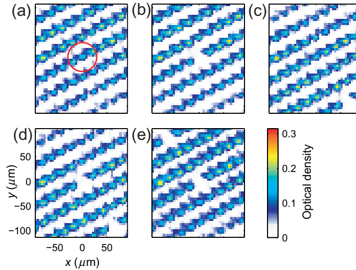
Figure 5. Single-site addressability and transport of an empty site. Sequence of images demonstrating single-site addressability using a focused laser pulse to empty a selected trap and transport using the atomic shift register. (a) Atoms are loaded to the lattice at a temperature of \sim 10 \mu\text{K} . The center of the red circle indicates the position of the focused addressing laser spot. (b) Optical pumping light focused on one lattice site is pulsed on for 1 ms to drive transitions to untrapped Zeeman states, completely emptying the microtrap. The effect of the addressing pulse on neighbouring traps is negligible. (c) All the traps along with the emptied site are shifted by three lattice periods to a new position (bottom right). (d) The addressing laser is pulsed on again to empty a second trap, and finally (e) the array is shifted back to the original position.
