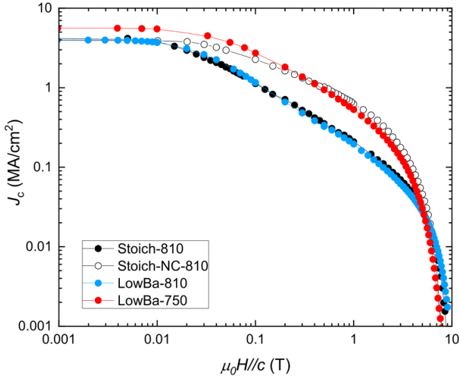
Figure 1. Critical current density values as a function of the applied magnetic field H/c at 77 K for samples: Stoich-810 (closed black dots), Stoich-NC-810 (opened black dots), LowBa-810 (closed blue dots) and LowBa-750 (closed red dots).
