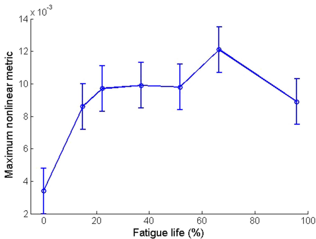
Figure 4. Maximum nonlinear metric, \gamma , as a function of % fatigue life (error bar represents an averaged standard deviation).
