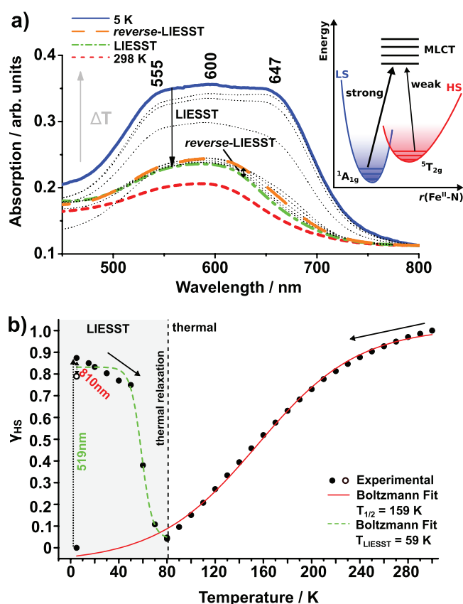
Figure 3. (a) Temperature-dependent UV/vis spectra of a vacuum-deposited film of compound [\text{Fe}(\text{4-me}_2\text{-bpz})_2(\text{phen})] on a quartz disk at 298 (red dotted line) and 5 K (blue line), and LIESST at 5 K (green line; 5 min at 519 nm) and reverse-LIESST at 5 K (orange line; 15 min at 810 nm). Gray traces show spectra taken during thermal relaxation (5 to 80 K) of the LIESST state. Inset: Ground and MLCT excited states and involved transitions. (b) High-spin fraction \gamma_{\text{HS}} versus T along with Boltzmann fit (red line). The light-induced SCO at 5 K is shown by dotted black arrows (green = LIESST and orange/red = reverse-LIESST), and thermal HS-to-LS relaxation is shown by a Boltzmann fit (green dotted line).
