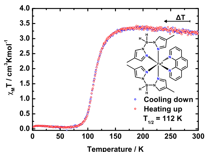
Figure 2. \chi_M T versus T curves of crystalline [\text{Fe}(\text{4-me}_2\text{-bpz})_2(\text{phen})] between 5 and 300 K. The curves resulting from cooling (blue symbols) and heating (red symbols) of the sample almost coincide. T_{1/2} was obtained from calculation and plot of \gamma_{\text{HS}}(T) (see SI, figure S4). Inset: Molecular structure of [\text{Fe}(\text{4-me}_2\text{-bpz})_2(\text{phen})] .
