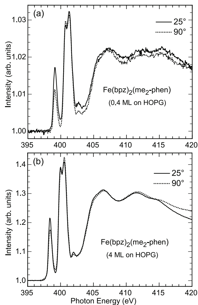
Figure 9. N K-edge spectra recorded at 25° (solid lines) and 90° (dots) angles between the x-ray beam and the HOPG surface of: (a) 0.4 ML of [Fe(bpz) 2 (me 2 -phen)]; (b) 4 ML of [Fe(bpz) 2 (me 2 -phen)].
