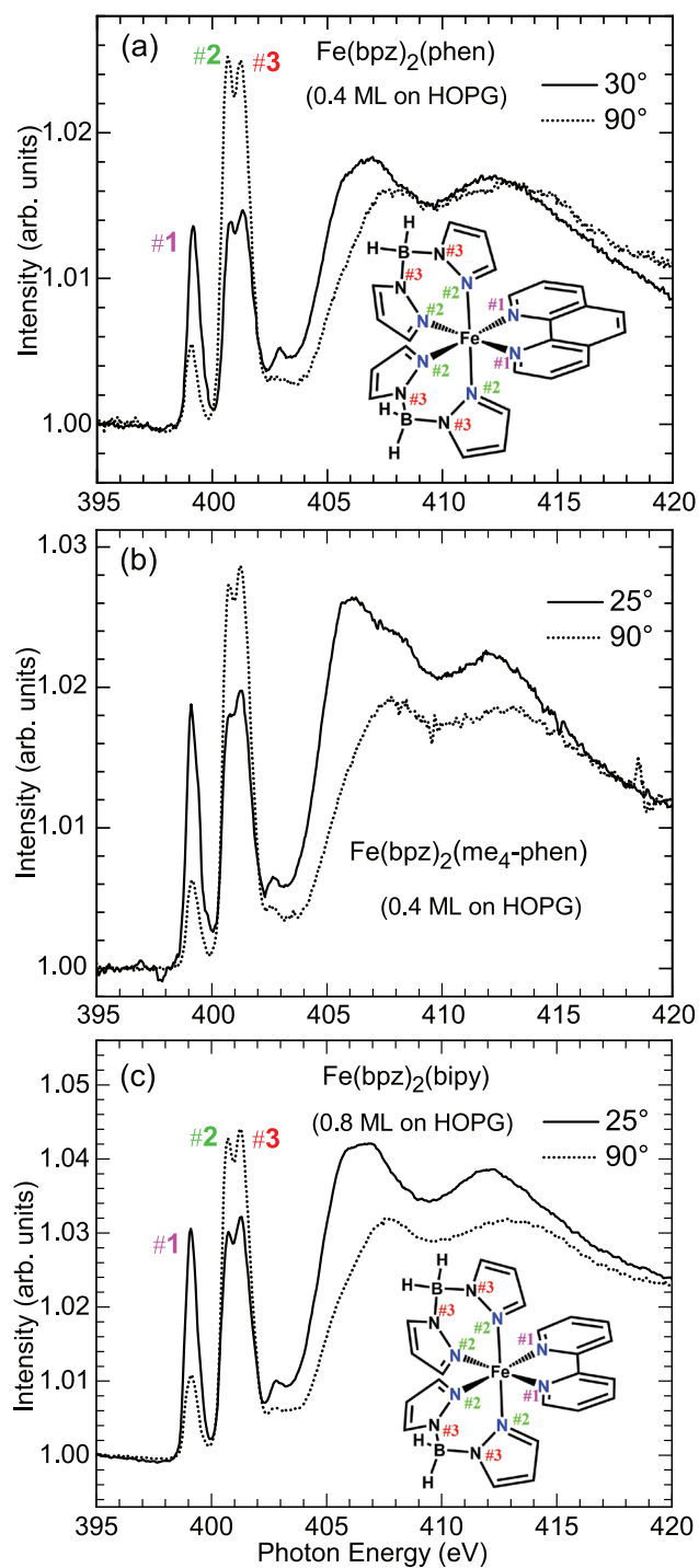
Figure 8. N K-edge spectra recorded at grazing (solid lines) and normal (dots) angles between the x-ray beam and the HOPG surface of: (a) 0.4 ML of [Fe(bpz) 2 (phen)]; (b) 0.4 ML of [Fe(bpz) 2 (me 4 -phen)]; and (c) 0.8 ML of [Fe(bpz) 2 (bipy)]. #1, #2 and #3 are the resonances corresponding to the N atoms as indicated in the inset.
