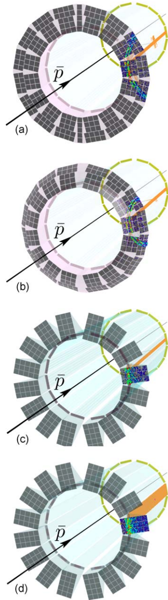
Figure 20. Geant simulation of the \bar{\text{PANDA}} Barrel DIRC using different design options. An oil tank with a straight (a) or curved (b) imaging plane is shown at the top. Solid fused silica prisms are used as EV in the design on the bottom (c), (d). Narrow bars (a)–(c) or wide plates (d) are used as radiator. Cherenkov photon trajectories from a 3 GeV/c kaon are shown in orange. The colored histogram shows the accumulated hit pattern from 100 kaons of the same momentum. Reprinted from [43], Copyright (2014), with permission from Elsevier.
