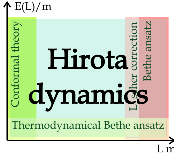
Figure 3. Domains of applicability of different descriptions of an integrable field theory at a finite volume L . In the ultra-violet regime, for small volume measured in units of a dynamically generated mass, the theory could be described by a conformal theory. In the infrared, at large volume, one can use the asymptotic Bethe equations. The leading order finite size corrections are governed by the (generalized) Lüscher corrections. At any volume but for the ground state energy only one can use Thermodynamical Bethe ansatz. Hirota equation, equivalent to Y-system but more efficient when it comes to imposing appropriate analyticity properties, is a universal tool covering the whole diagram.
