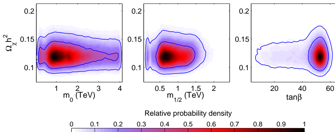
Figure 6: The 2-dim relative probability density p(\Omega_\chi h^2, \theta_i | d) , where \theta_i = m_0, m_{1/2} and \tan \beta . Note that the measured value of \Omega_\chi h^2 , eq. (3.10), has been included in computing the relative probability density.
