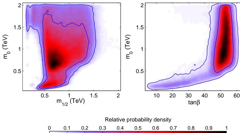
Figure 3: The 2-dimensional relative probability densities as in figure 2 but for the “2 TeV range” analysis and for the planes (m_{1/2}, m_0) and (\tan\beta, m_0) only. Imposing a prior range m_0 < 2 TeV modifies substantially the inferences about the high probability regions for m_0 .
