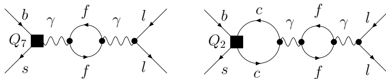
Figure 3: Vacuum polarization diagrams.
