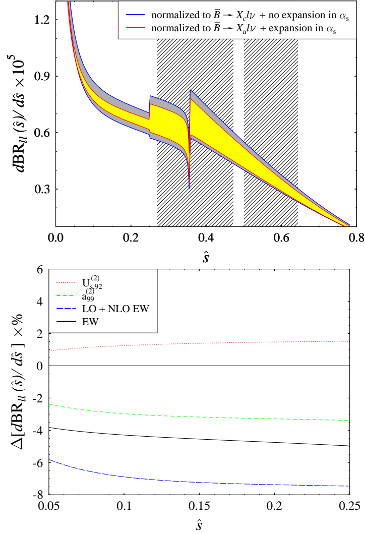
Figure 5: Scale dependence of the differential \text{BR}_{\ell\ell} using the different normalizations of eqs. (4.1) and (4.4) in the partial NNLO QCD approximation (upper plot). The discontinuity at the end of the low- \hat{s} region reflects the fact that the O(\alpha_s^2) matrix elements of Q_1 and Q_2 have not been implemented for \hat{s} > 0.25 [8], while the divergence in the J/\psi region is due to the 1/m_c^2 corrections. Furthermore the relative size of the NNLO and electroweak (EW) effects introduced in this paper are shown when sequentially included (lower plot).
