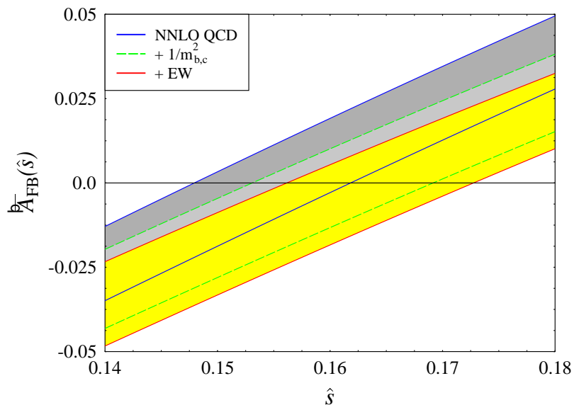
Figure 7: Normalized FB asymmetry \bar{A}_{FB}(\hat{s}) in the low- \hat{s} region in the NNLO QCD approximation as given in eq. (4.10) without expansion in \alpha_s . Furthermore the effects of including power corrections (central band) and higher order electroweak effects (lower yellow band) are shown.
