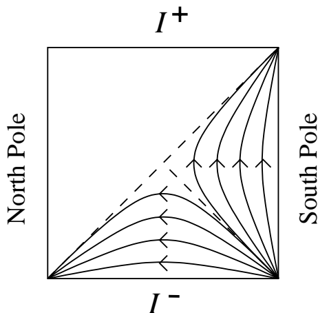
Figure 3: The arrows indicate the direction of the Killing flow generated by L_0 + \bar{L}_0 within \mathcal{O}^- . Note that it is timelike along the worldline of an observer at the south pole but becomes spacelike on \hat{\mathcal{I}}^- .
