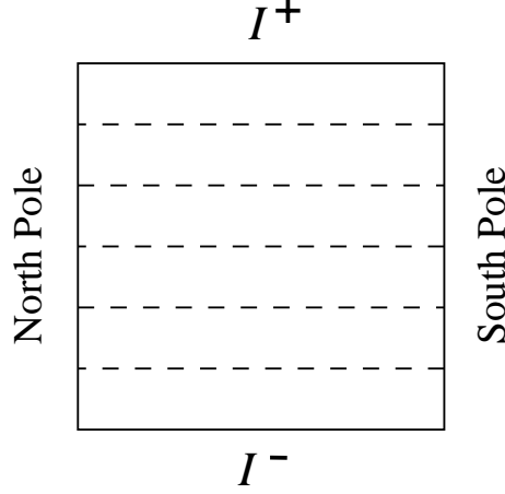
Figure 2: Lines of constant \tau in global spherical coordinates are the spacelike two-spheres indicated by dashed lines.
