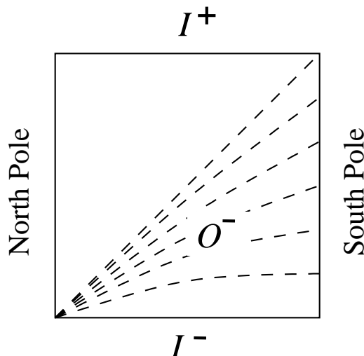
Figure 1: Penrose diagram for dS_3 . Every point in the interior of the diagram is an S^1 . A horizontal line is an S^2 , with the left (right) vertical boundary being the north (south) pole. O^- is the region below the diagonal, and comprises the causal past of an observer at the south pole. The dashed lines are non-compact surfaces of constant t .
