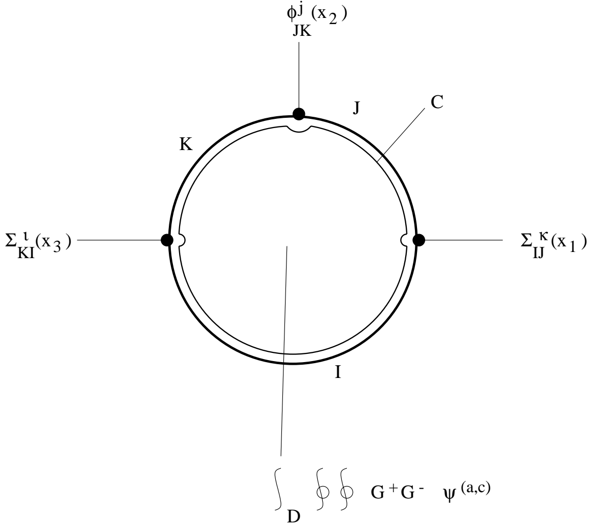
Figure 2: Perturbation of cubic part of superpotential by Kähler deformation. The superconformal Ward identities allow us to pull \oint dz G^+(z) to the contour C . This can be deformed to a contour integral around each of the boundary operators and an integral over C of d\bar{z} \bar{G}^+(\bar{z}) which can be deformed back to the insertion of \bar{G}^- \psi . The result is an integral over the insertion of \bar{\partial}_w \psi which can be integrated by parts to an integral of \psi over C .
