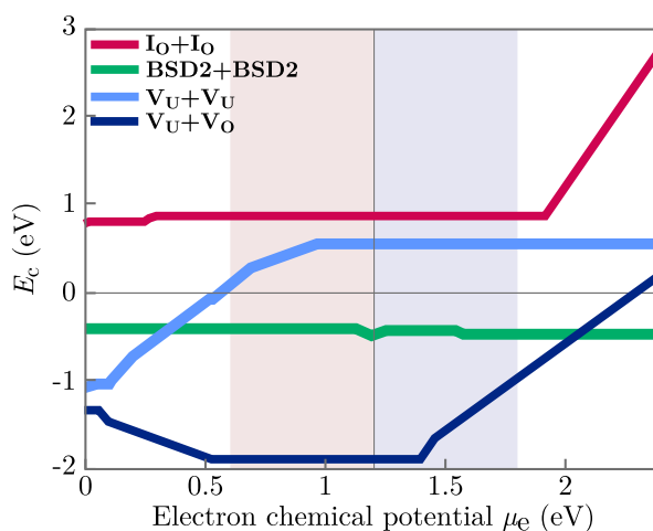
Figure 7. Clustering energies of the I_2^X (red), Di-Schottky (green), 2V_U (light blue) and V_U V_O (dark blue) clusters.
