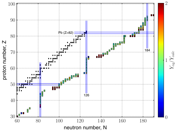
Figure 7. Comparison of abundances from our calculations with (n,\gamma) – (\gamma,n) equilibrium abundances on the r -process path for the FRDM mass model. The colors show the factor Y_{\text{eq}}/Y_{\text{calc}} . Only the most abundant nuclei are shown for each isotopic chain. See the text for details.
