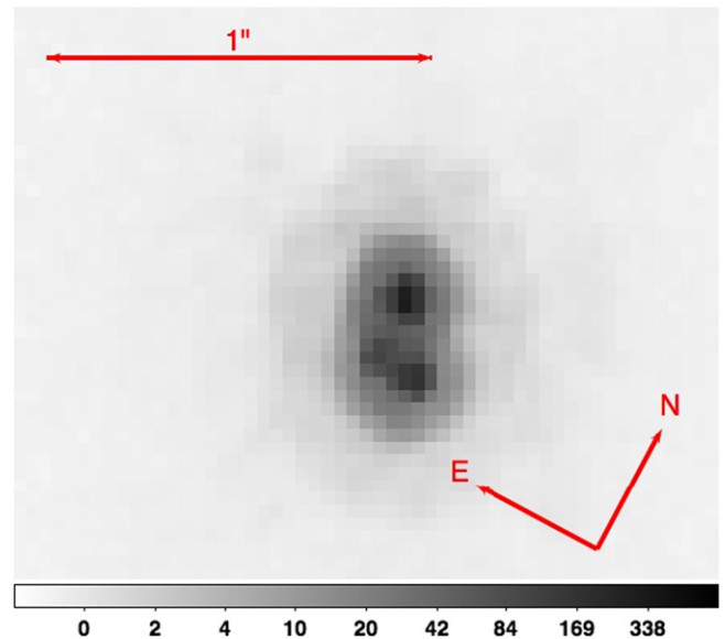
Figure 4. Drizzled image of KOI-2626 in the F775W filter showing a 1".0 scale bar and orientation. Component B is lowest in the image, with component C to the left. The scale and units are the same as in Figure 1. The FWHM of the PSF is 0".3870 for the blended system.
