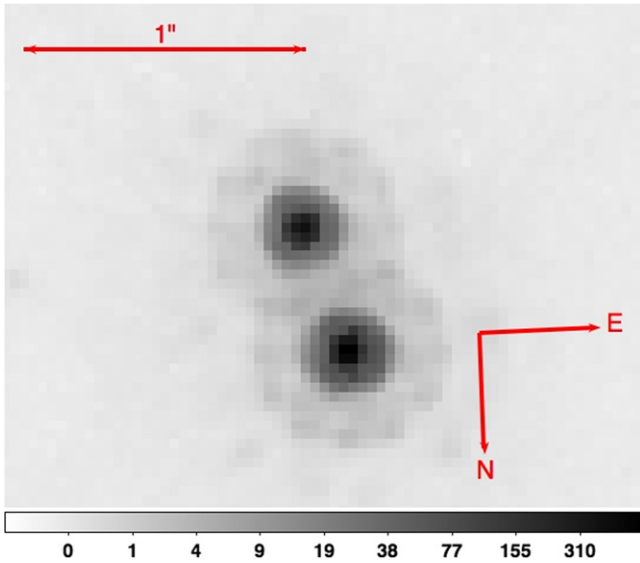
Figure 5. Drizzled image of KOI-3049 in the F775W filter showing a 1'' scale bar and orientation. The fainter component, B, is toward the top. The scale and units are the same as in Figure 1. The FWHM of the PSF is 0''.5563 for the blended system.
