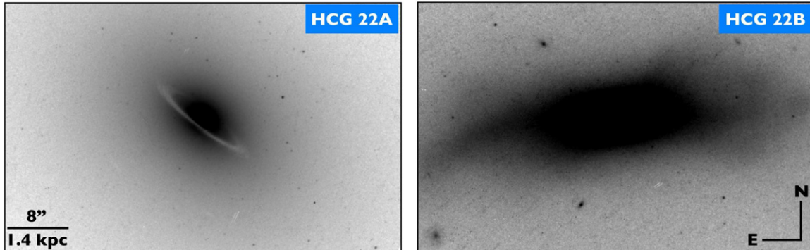
Figure 9. Left: a prominent dust lane can be seen in this HST -F450W image of the inner ∼2 kpc of HCG 22A, possibly the signature of a recent merger. North is to the top and east to the left of the image, as is the image on the right, where the contrast of the F814W frame has been set to demonstrate the various disturbances in the optical morphology of HCG 22B. We interpret this as the result of a recent merger (following a series of passages).
