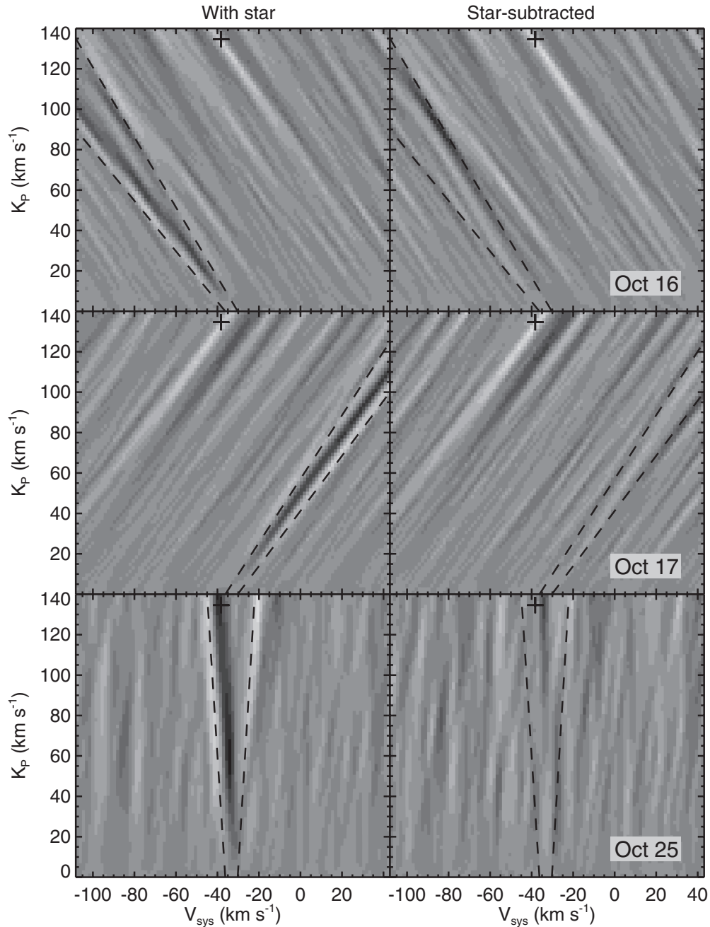
Figure 2. Left column: total cross-correlation signal for each night of observations, without removing the stellar absorption lines. Right column: same as the left column, but after removing the stellar spectral features. In all panels, a linear color scheme running from -7\sigma (black) to +7\sigma (white) is adopted. The crosses indicate the planet position measured by combining the nights of October 16 and 17. The black-dashed lines encompass regions of the parameter space significantly affected by stellar residuals. These result in extra cross-correlation noise, potentially masking the planet signal in the third night, as discussed in Section 4.1.
