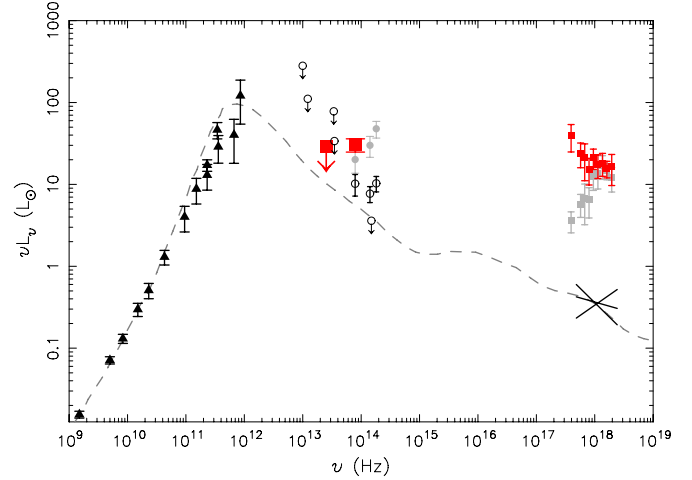
Figure 5. SED of Sgr A*: in black (filled triangles) are radio to submillimeter measurements of the quiescent state (Markoff et al. 2001; Zhao et al. 2003). Note that these measurements are time-averaged measurements and the error bars include variable emission of up to 50%. As open black circles with arrows are shown 30 \mu\text{m} , 24.5 \mu\text{m} , and 8.6 \mu\text{m} upper limits taken from Melia & Falcke (2001), the upper limit at 8.6 \mu\text{m} from Schödel et al. (2007) and the limit on the quiescent state at 2 \mu\text{m} from Hornstein et al. (2002). The quiescent state values from Genzel et al. (2003) are shown as the open black circles with error bars, and the flare values from the same paper as gray filled circles. The X-ray quiescent state is shown as the black bow-tie (Baganoff et al. 2003). The dashed line shows a model for the quiescent state (Yuan et al. 2003). Our new measurements for the SED of a flaring state of Sgr A* are shown in red (filled squares): (1) the MIR ( 11.88 \mu\text{m} ) upper limit is shown as the downwards-pointing arrow. The MIR upper limit is determined over an interval 05:30 to 06:13 (see the discussion in Section 2.3). (2) The L'-band measurement is shown as the red square with error bars. This corresponds to extinction corrected, background subtracted mean value of the L'-band observations, 19.1 \pm 3.6 \text{ mJy} (in this case we used the minimum of the light curve, 2.4 \text{ mJy} as the background estimate). Since the MIR observations did not start until 5:30 (approximately half an hour after the onset of the NIR flare), the mean was computed over the MIR time interval rather than the entire L'-band flaring interval. Also shown next to the L'-band data point is how the L'-band measurement would continue into Ks and H bands with a slope of 0.4, characteristic of the L'-H slope of a number of “bright” observed flares in the literature (Hornstein et al. 2007; Gillessen et al. 2006) and also consistent with the slope of the peak flare values of Genzel et al. (2003). (3) Two possible X-ray spectra are shown, neither of which is model-independent. The red points which slope upwards to the left indicate the power-law fit, of Porquet et al. (2008), while the gray points show the blackbody fit of the same paper. The X-ray spectrum was scaled by a small factor since it incorporated data from an extra five minutes before the MIR observations began.
