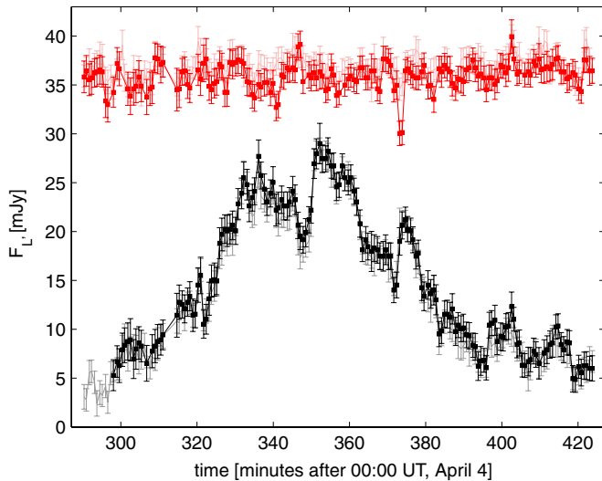
Figure 2. Extinction-corrected L' -band flux of Sgr A* on 2007 April 4, determined via PSF photometry (black data points) and via aperture photometry (gray data points). Above the light curve of Sgr A* is shown in red (PSF photometry) and light red (aperture photometry) the flux of the nearby star S2 as a flux comparison, clearly demonstrating that the substructure is intrinsic to the Sgr A* source. S2 was confused at the time of observation with S13, and in the figure their combined flux is shifted upwards by 25 mJy. Sgr A* was confused with S17 and the flux shown also possibly has a contribution from a dust cloud as well as the unknown quiescent state of Sgr A*. The data are binned to a bin-width of 44.3 s. The PSF photometry method only lists fluxes of sources detected with 3\sigma significance, which explains why the light curve derived by PSF photometry begins only at around \sim 300 minutes. We use the mean of these points with t \lesssim 300 minutes as an upper estimate of the background level (S17 + confused sources + quiescent state) upon which the flare emission is superimposed. If the minimum of the light curve is used instead, we obtain a background estimate of 2.4 mJy.
