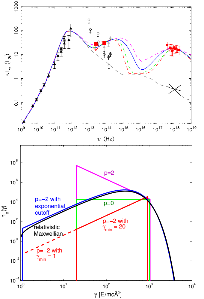
Figure 8. Upper panel: best-fit SEDs where the NIR synchrotron emission is produced by a power-law distribution of electrons with index p = 2, 0, -2 (magenta, green, and red dashed lines). The best-fit model for a thermal distribution of electrons is shown in solid blue. All models appear relatively similar. Note that the (model-dependent) X-ray data are only shown for the thermal distribution of electrons case, but it should be similar for the other models. Lower panel: the electron energy distributions of best-fit submillimeter IC models each assuming a different underlying form for the energy distribution. We compare power-law models ( n(\gamma) \propto \gamma^{-p} ) of index p = 2, 0 , and -2 (magenta, green, and red, respectively). We also demonstrate that in a power-law model of index -2 with an exponential cutoff (blue) we found the same energy distribution as in the thermal distribution case (in black; note that we used analytical equations to calculate the synchrotron emission for the thermal case in icmodel and sscmmodel of Section 4). Although the electron distributions all look very different, they all cross at an energy \gamma \approx 1000 .
