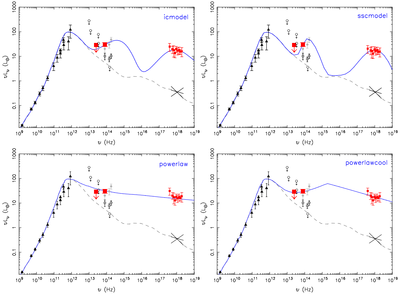
Figure 6. Best fits of the four XSPEC models for the April 4 flare IR and X-ray data. The X-ray data points are the unfolded spectrum for the given model (blue solid line); only the PN unfolded spectra are shown, with the data points binned for plotting purposes. (1) icmodel : the solid blue line shows the best-fit IC model for the fit constraints of the April 4 flare, which satisfies the MIR limit and the NIR spectral index. The dashed blue line shows the best-fit model holding the magnetic field fixed at B = 30 G. This model violates the NIR spectral index and comes close to violating the MIR upper limit. It does however allow a larger size for the quiescent region, R_Q = 0.27R_S . This is however still far from the size/photon densities expected from size measurements of Sgr A*. (2) sscmmodel : best-fit SSC model. In this case the magnetic field and density are extremely high. The source becomes self-absorbed in the NIR, and the spectrum shows strong curvature from L' to H band. (3) powerlaw : best-fit power-law model. This model violates both MIR limit and NIR spectral index. (4) powerlawcool : a more feasible synchrotron model with a cooling break. This model corresponds to the steady state solution for a system with a constant injection of power-law electrons where the energy loss of the electrons due to synchrotron emission is taken into account.
