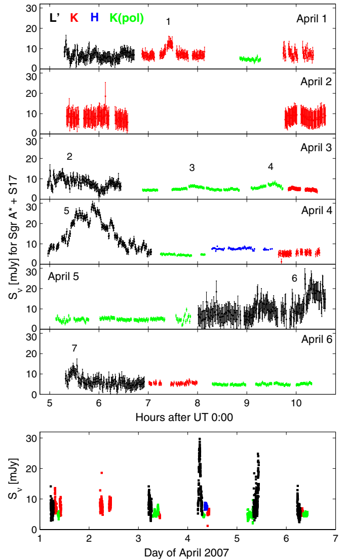
Figure 1. Light curve for Sgr A* + S17 for 2007 April 1–6 IR/NIR observations with NACO at the VLT. Observations were taken at L' (black), Ks (red), H (blue), as well as in Ks band using polarimetric mode (green). Several flare events are seen over the six nights of observations, labeled 1–7. Some nights show a more continuous level of variability (April 3), while on other nights there are long periods with no obvious variable emission. The L'-band flare from April 4 is the most significant event seen. A flare of equivalent strength in Ks band (given a color of \beta = 0.4 in \nu L_\nu ) would reach S_K \sim 20 mJy. On April 5, another L'-band flare is seen under less favorable conditions which reaches S_{L'} \sim 20 mJy in L' band.
