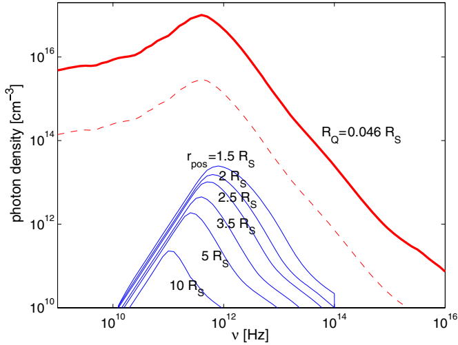
Figure 7. Comparison of the photon density at each frequency in (i) the best-fit IC model with R_Q = 0.046 R_S (thick red solid line) and (ii) different radii between 1.5 R_S and 10 R_S in the Yuan et al. (2003) model (thin blue solid lines). The dashed red line shows the photon density spectrum for R_Q = 0.27 , at the 90% confidence level for the parameter R_Q . The photon densities of Yuan et al. (2003) are in general 2–3 orders of magnitude too low, which shows why there is no well fitting IC model for the multiwavelength observations of the April 4 flare, given the photon densities of the Yuan et al. (2003) model.
