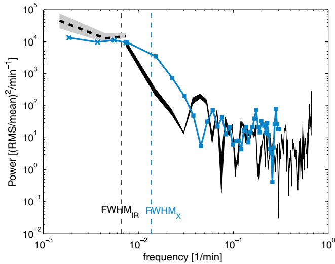
Figure 4. Power spectra of the L'-band (thick black) and X-ray (blue squares) light curves. Our constraint on the periodogram at low frequencies from Ks and H-bands data is shown as the gray region (with the interval mean shown as black dashed line). The rms-squared normalization was used, where the mean of the IR and X-ray light curves was taken from the same time interval. A peak is seen around the 20 minute timescale ( \sim 0.04 \text{ minute}^{-1} ), while there is no corresponding peak in the X-ray power spectrum. The two dashed lines indicate the corresponding FWHM frequency for the Fourier transform of a Gaussian given the FWHM durations of the IR and X-ray flares.
