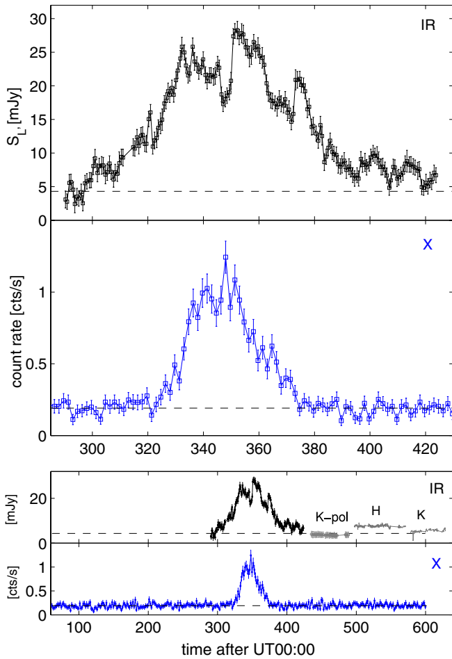
Figure 3. Comparison of the L' band and 2–10 keV light curves (labeled IR and X, respectively). The top two panels show the two flares over the period of the L' -band observations. In the lower two panels, a larger time interval is shown. We also show data taken in other wavelength bands (Ks-band polarimetry, H-band imaging, and Ks-band imaging) subsequent to the L' -band flare indicating that the flare activity ceased in both wavelength bands after roughly 4:00 UT. In the same night of observations three more X-ray flares were seen (Porquet et al. 2008); the first of these started at UT 11:32 (692 minutes), i.e., roughly an hour after the last of the NIR observations. The dashed lines indicate our estimates of the background levels (i.e., emission that is not flaring emission) at each wavelength. In the case of the IR light curve this may be an overestimate. (A color version of this figure is available in the online journal.)
