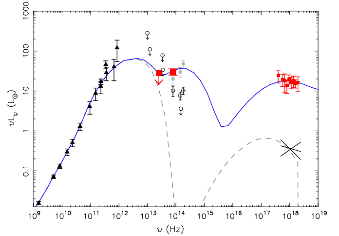
Figure 9. Submillimeter inverse Compton model for the X-ray flare using a different model (the jet model; Falcke & Markoff 2000) as template for the submillimeter photon spectrum. The dashed gray line shows the jet model which is used as the source of seed photons. The solid blue line shows the best-fit XSPEC model.
