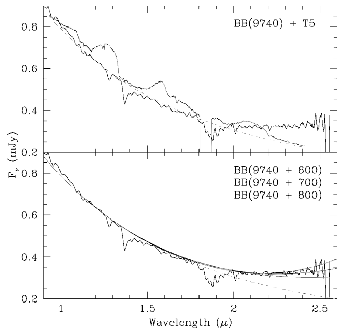
FIG. 4.—GD 362 spectrum (black line) and the expected infrared flux from a blackbody (BB) at 24 pc (dashed line). Composite blackbody + brown dwarf/blackbody templates are shown as gray lines in both panels. The bottom panel shows the effect of changing the temperature of the secondary blackbody from 600 to 800 K (from top to bottom). [See the electronic edition of the Journal for a color version of this figure.]
