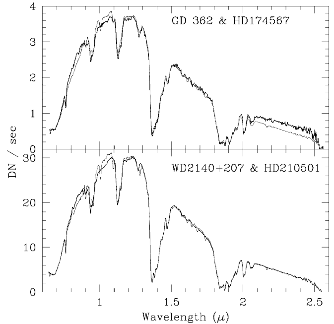
FIG. 2.—Uncalibrated spectra of GD 362 and its reference A0 V star (top panel) and of WD 2140+207 and its reference A0 V star (bottom panel). The spectra for white dwarfs are shown in black, whereas the spectra for A0 V stars are shown in gray. [See the electronic edition of the Journal for a color version of this figure.]
