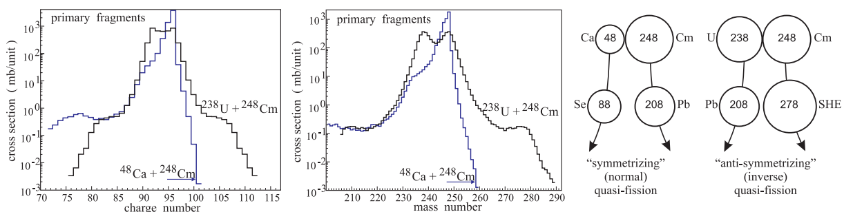
Figure 8. Charge and mass distributions of heavy primary reaction fragments formed in collisions of ^{238}\text{U} and ^{48}\text{Ca} with ^{248}\text{Cm} target at E_{\text{c.m.}} = 750 and 220 MeV, correspondingly. Schematic view of “normal” and “inverse” quasi-fission processes are also shown.
