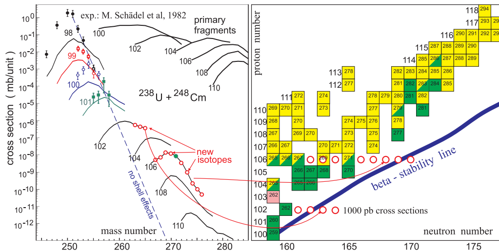
Figure 9. Yield of survived isotopes of SH nuclei produced in collisions of ^{238}\text{U} with ^{248}\text{Cm} target at E_{\text{c.m.}}=750 MeV. New isotopes of nobelium and seaborgium are shown by open circles.
