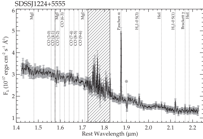
Figure 2. LBT LUCI-1 near-infrared spectrum of the nuclear source corrected for redshift, with labels for features detected. Also noted is a strong telluric absorption feature at 1.9 \mu\text{m} from imperfect telluric corrections, indicated by the encircled plus line. The diagonally hatched lines note a region of strong absorption due to Earth's atmosphere.
