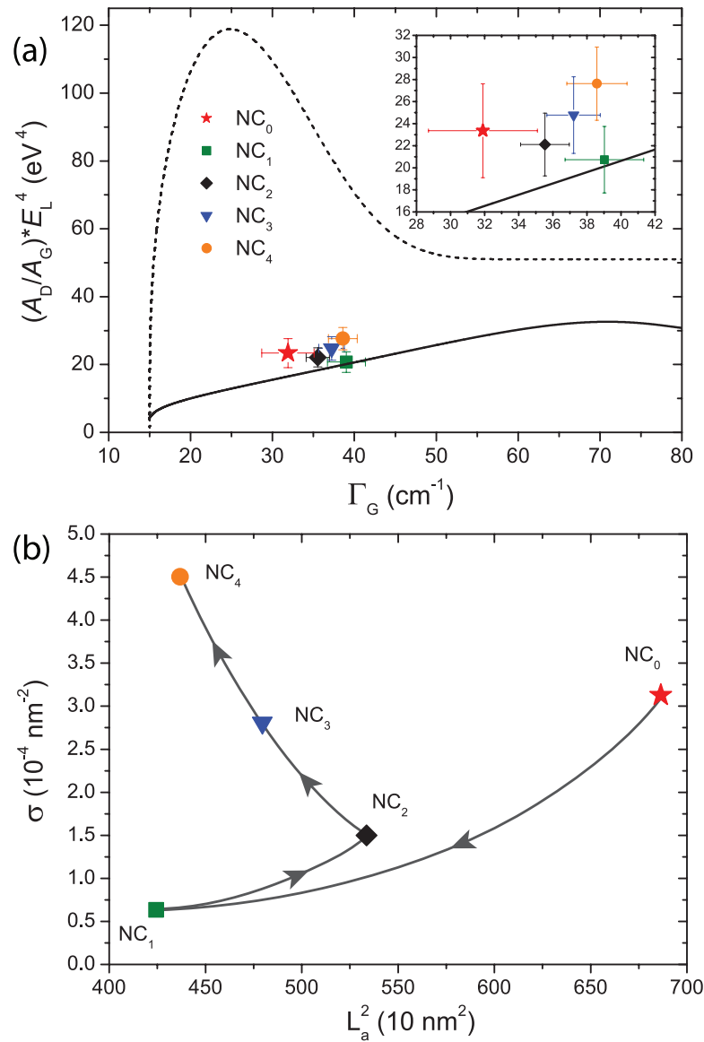
Figure 4. Characterization of graphene-related samples produced by the cracking of a methane/CO 2 mixture into graphitic carbon and hydrogen via the cold microwave plasma method. [40] The five distinct samples were produced by setting different initial CO 2 contents, namely 0% (NC 0 ), 0.4% (NC 1 ), 1.7% (NC 2 ), 4.9% (NC 3 ) and 7.4% (NC 4 ). (a) (A_D/A_G)E_L^4 as a function of \Gamma_G . Data points correspond to average values extracted from 1681 spectra taken from different regions in each sample. The lengths of the error bars resemble the standard deviation. The solid and dashed lines are the same as in figure 3, reproduced here for reference. The inset is a zoom within the experimental data. (b) Plot of the defect density ( \sigma = 1/L_D^2 ) versus crystallite area ( L_a^2 ), with the respective ( L_a , L_D ) values are extracted from figure 3. Exemplary Raman spectra can be found in [40].
