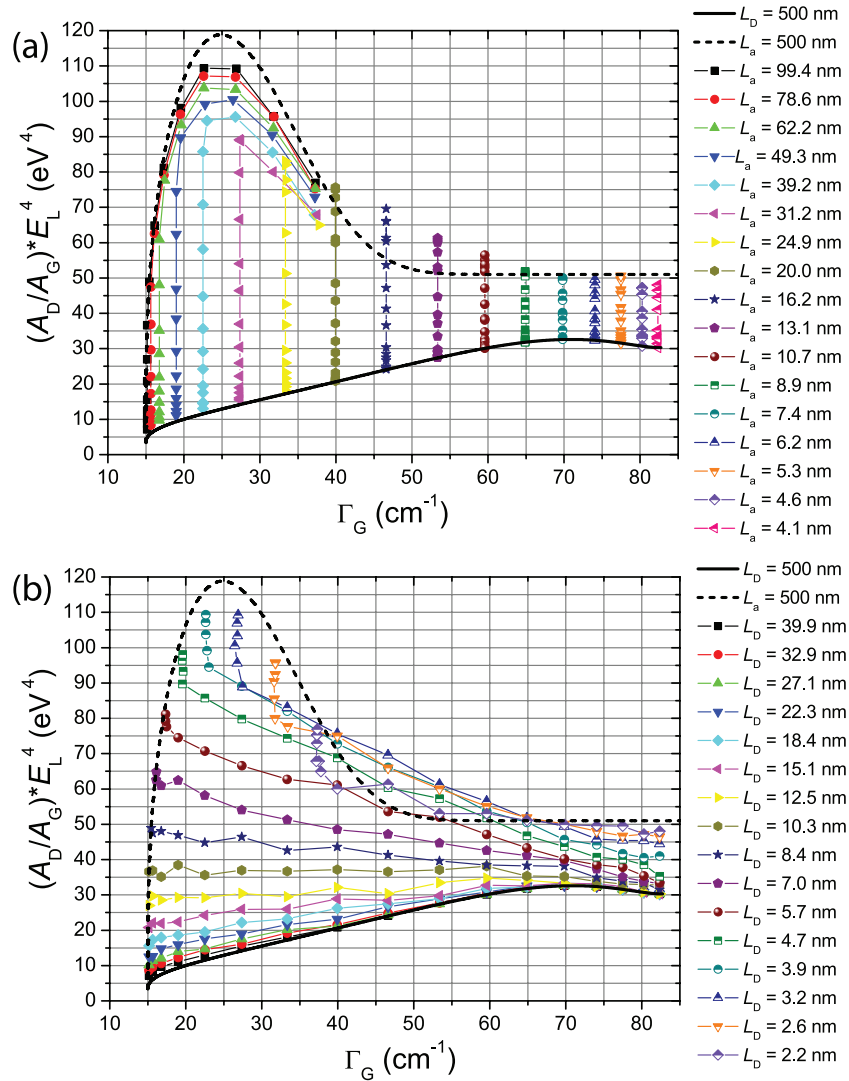
Figure 3. Theoretical calculation for the (A_D/A_G)E_L^4 as a function of the G band spectral linewidth \Gamma_G . The symbols were obtained from numerical simulations (see text). In (a), equal symbols connected by lines represent samples with a given L_a value (indicated in the legend), with decreasing L_D distances from smaller to larger \Gamma_G values. (b) The opposite: equal symbols connected by lines represent samples with a given L_D value (indicated in the legend), with decreasing L_a distances from smaller to larger \Gamma_G values. The dashed lines in (a) and (b) are the same plot of (A_D/A_G)E_L^4 as a function of \Gamma_G obtained from equations (4) and (1), respectively, by varying L_D and considering a fixed value of L_a = 500 nm. The solid lines correlate (A_D/A_G)E_L^4 with \Gamma_G (obtained from equations (4) and (1), respectively) for different values of L_a , with L_D fixed at 500 nm.
