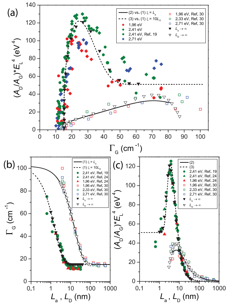
Figure 2. Spectral behavior for the amorphization routes in graphene materials. (a) (A_D/A_G)E_L^4 as a function of \Gamma_G . The solid line is a plot of the one-by-one correlation between the values obtained from equation (1) (with \xi = L_a ) and (2), for L_a ranging from 4 to 1,000 nm in steps of 0.01 nm. Similarly, the dashed line correlates the values obtained from equation (1) (with \xi = 10L_D ) and (3), for L_D ranging from 0.01 to 1,000 nm in steps of 0.01 nm. (b) \Gamma_G as a function of L_a and L_D , separately. The solid and dashed lines are the plots of equation (1) as a function of L_a ( \xi = L_a ) and L_D ( \xi = 10L_D ), respectively. (c) (A_D/A_G)E_L^4 as a function of L_a and L_D , separately. The solid and dashed lines are the plots of equations (2) and (3) as a function of L_a and L_D , respectively. In all panels, filled and open symbols represent samples with point- and line-defects, respectively. Same definition for dashed and solid lines, respectively. The value of E_L for each experimental data set is displayed in the legends, in eV units. The data represented by diamonds in (a) were generated for this work. The bullets and open squares were extracted from [19] and [30], respectively. The filled up-triangles were taken from [24]. The empty and filled down-triangles are data obtained from numerical simulation with L_a \rightarrow \infty and L_D \rightarrow \infty , respectively. Exemplary Raman spectra can be found in appendix A.
