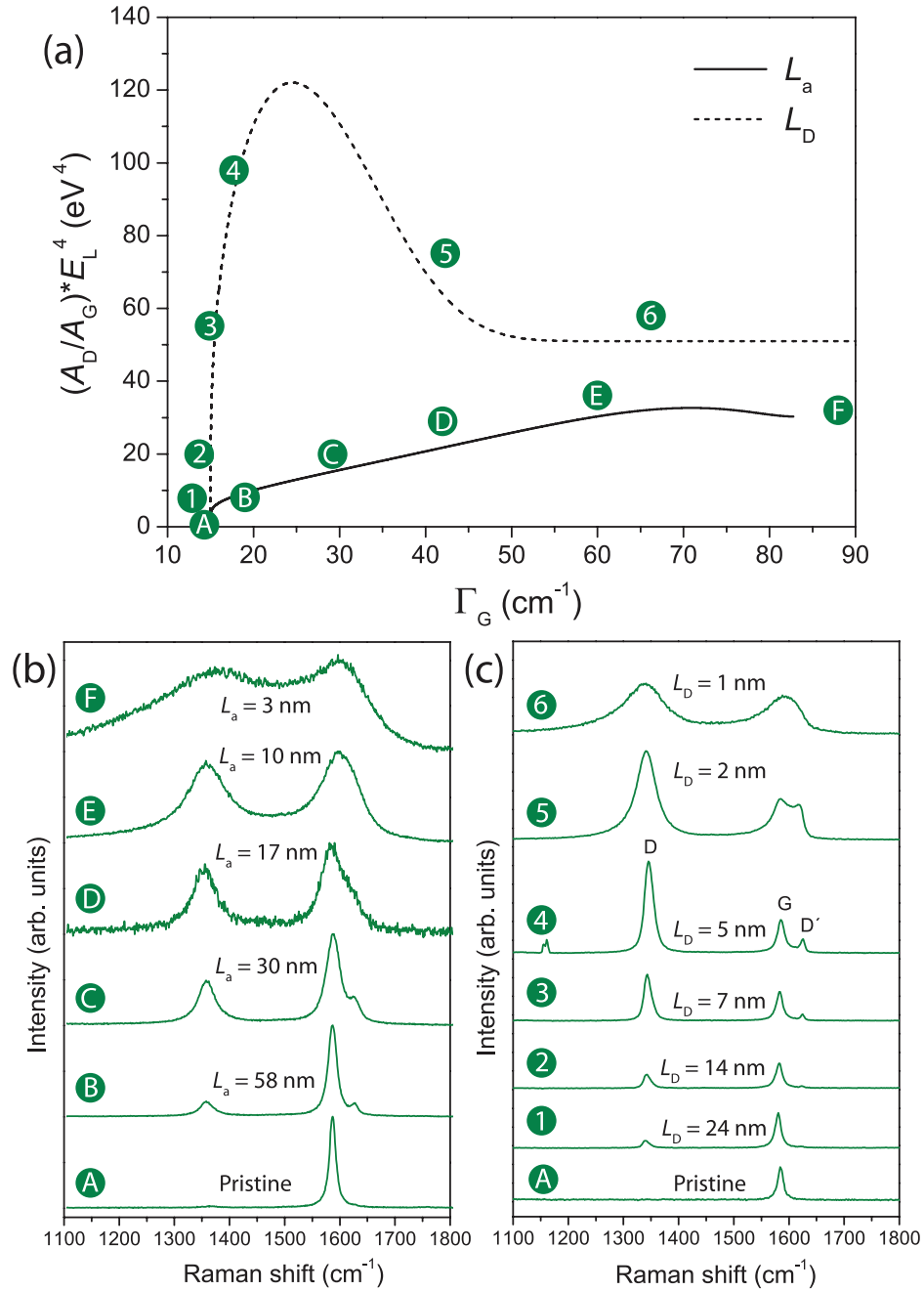
Figure A1. Exemplary Raman spectra within the Raman phase diagram of figure 2. (a) Reproduces the (A_D/A_G)E_L^4 as a function of \Gamma_G theoretical diagram (lines), showing only the experimental data points related to the Raman spectra shown in (b) and (c). (b) Exemplary Raman spectra for samples following the amorphization route of pure line defects. (c) Exemplary Raman spectra for samples following the amorphization route of pure point defects. The letters/numbers correlate the specific spectrum in (b)/(c) with the spectral location at the Raman phase diagram in (a).
