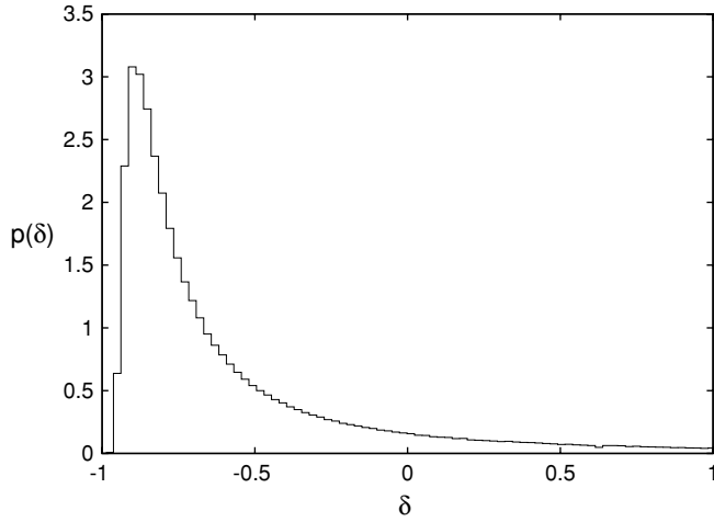
Figure 1. One-point PDF of our density field, sampled with a spherical top-hat window function of radius 1 h^{-1} Mpc.
