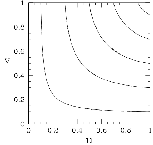
Figure 2. Empirical two-point copula C(u, v) for a simulated dark matter density distribution at a separation of 2 h^{-1} Mpc. Solid curves are the contours corresponding to (from lower left to upper right) C(u, v) = 0.1, 0.3, 0.5, 0.7, 0.9 . Dashed curves give the Gaussian copula with the value of r corresponding to Spearman's \rho calculated for the data.
