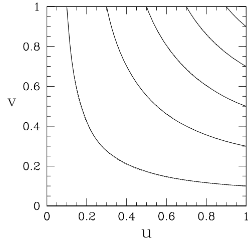
Figure 3. As Figure 2, for a separation of 6 h^{-1} Mpc.
