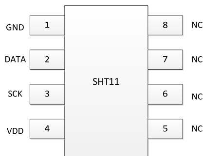
Figure 4. Pin diagram
