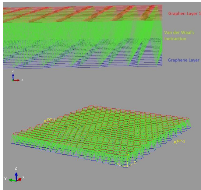
Figure 4. Double Layered Graphene Model
