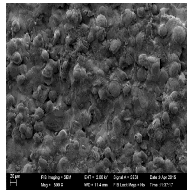
Figure 2. SEM image of \text{Al}_2\text{O}_3 -40% \text{TiO}_2 coated substrate
