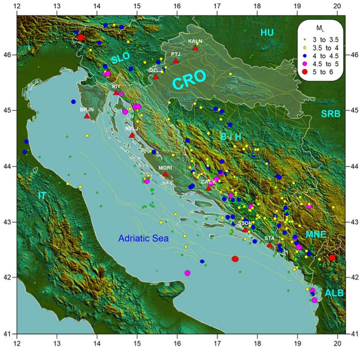
Figure 1. Map of earthquake epicentres (2002-2016) used in this study ( M_L \geq 3 , R_E \leq 150 km, and h < 30 km). Locations of seismic stations are marked with red triangles. Yellow lines represent known surface faults in Croatia and Bosnia and Herzegovina [6]
