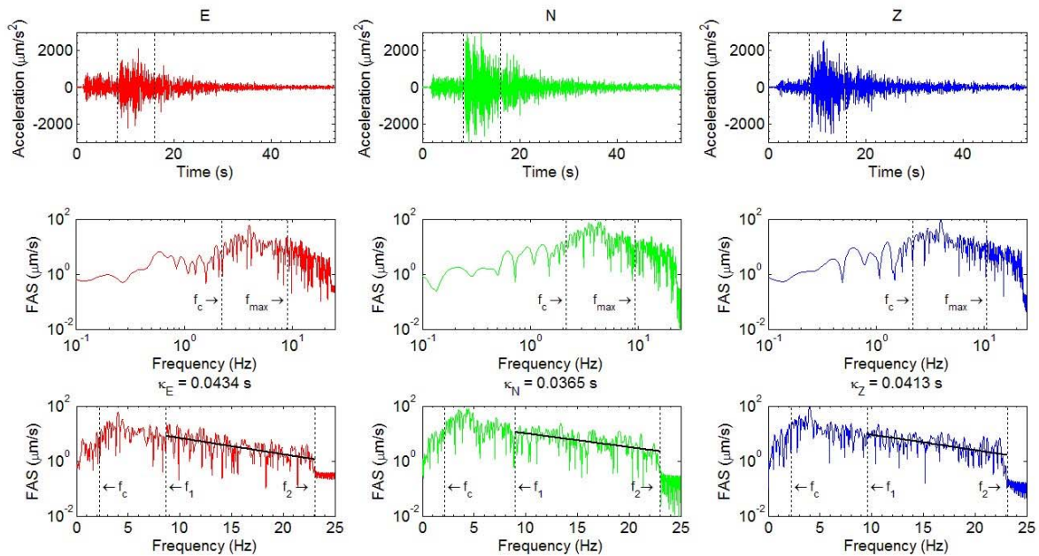
Figure 2. Example of kappa calculation using AH84 method for three components ( E , N , and Z ) seismogram. Station RIY, earthquake event on 16th June 2013 at 20:04, M_L=3.8 , R_E=56 km
