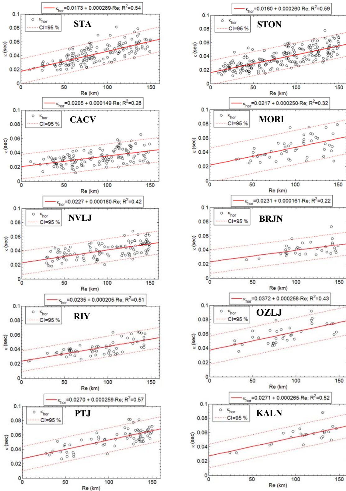
Figure 3. \kappa_{hor} model for Croatia as a function of a site (seismic station) and epicentre distance using standard linear regression (thick red line) with confidence interval (CI) of 95% (dashed line).
