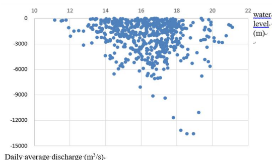
Figure 2. Daily average discharge of Hukou Station before jump alteration.
