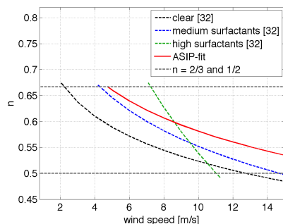
Figure 1. The Schmidt number exponent n versus wind speed based on Krall [38] for high surfactant coverage (0.26 mmol/l Triton in green), medium surfactant coverage (0.052 mmol/l Triton in blue), clean surface (black), and the best fit between the measured \epsilon and k_{DMS} in the small-eddy model during Knorr11 (red). The grey colored lines give the theoretical boundaries of n = 1/2 and n = 2/3 .
