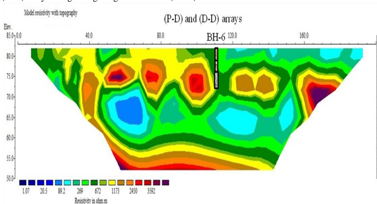
Figure 5: The model resistivity result for Bukit Bunuh area subsurface characterization using (P-D) and (D-D) arrays along with geological reference (BH-6).
