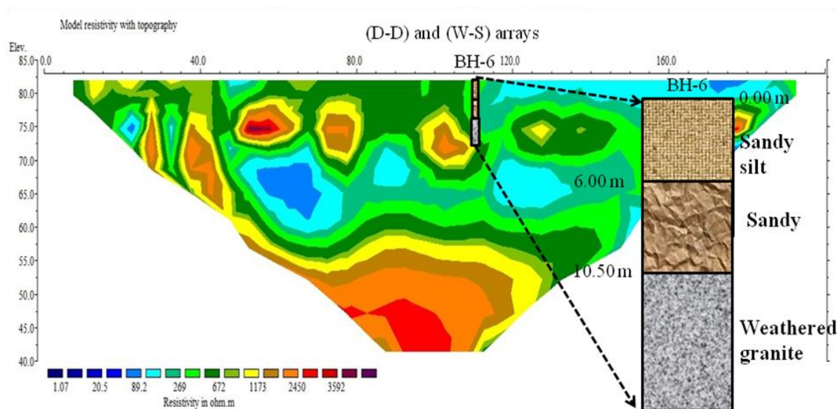
Figure 4: The model resistivity result for Bukit Bunuh subsurface characterization using (D-D) and (W-S) arrays along with geological reference (BH-6).
