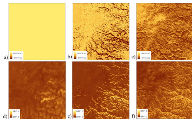
Figure 4. Comparison of the topographic correction at different level. (a) Irradiance with no topographic correction ( \text{W.m}^{-2} ), (b) Corrected irradiance at pixel level ( \text{W.m}^{-2} ), (c) Corrected irradiance at sub-pixel level ( \text{W.m}^{-2} ), (d) Surface reflectance with no topographic correction, (e) Corrected surface reflectance at pixel level, (f) Corrected surface reflectance at sub-pixel level.
