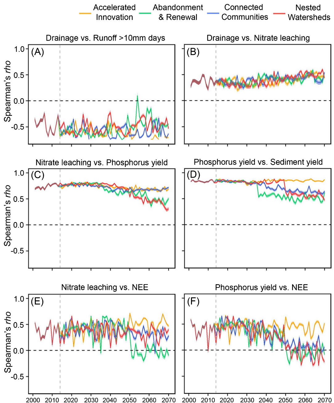
Figure 6. Changes in relationships among water and biogeochemical services at the grid-cell scale from 2001–2070 under four future scenarios. Scenarios were color-coded, with thick color lines as Spearman correlation coefficient and color ribbons as 95% confidence interval, on the basis of bootstrap approach with 1000 iterations.
