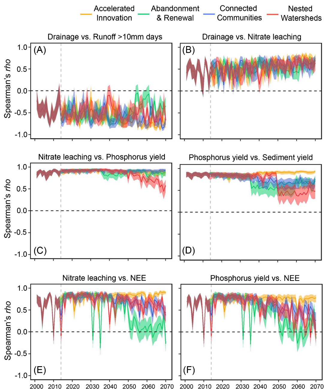
Figure 7. Changes in relationships among water and biogeochemical services at the subwatershed scale from 2001–2070 under four future scenarios. Scenarios were color-coded, with thick color lines as Spearman correlation coefficient and color ribbons as 95% confidence interval, on the basis of bootstrap approach with 1000 iterations.
