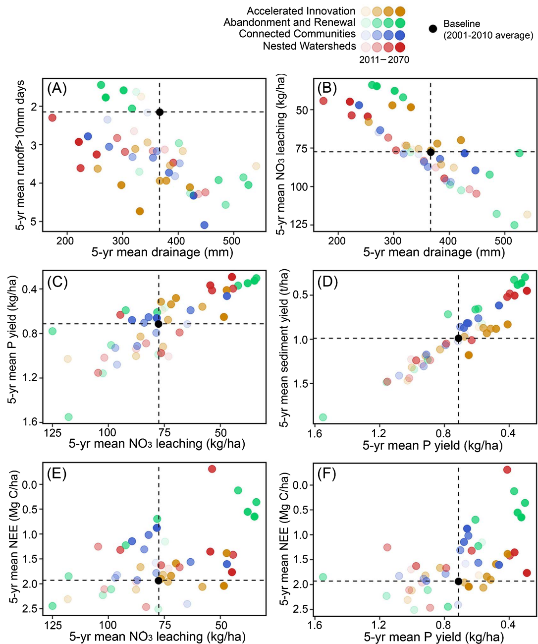
Figure 8. Changes in relationships among water and biogeochemical services at the watershed scale from 2001–2070 under four future scenarios. Scenarios were color-coded, and temporal changes in the indicators of paired services were calculated at the watershed scale at 5 year intervals (i.e. 2011–2015, 2016–2020...2066–2070). For a given scenario (colored circle), the gradient from lightest to darkest represents the time dimension from 2011–2015 to 2066–2070. Solid black circles are the baseline estimates (averaged 2001–2010) for comparison. Please note that y -axes were reversed for services quantified using inverse indicators.
