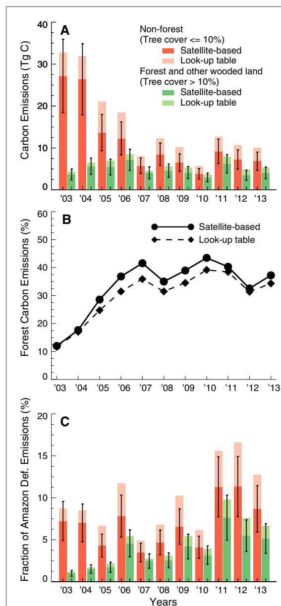
Figure 3. (a) Satellite-based and look-up table estimates of annual gross carbon emissions from cropland expansion into non-forest (orange) and forested (green) Cerrado cover types between 2003 and 2013. Error bars indicate \pm average uncertainty in satellite-based vegetation carbon stocks within cropland expansion areas. (b) Fractional contribution of forest conversion to gross carbon emissions from cropland expansion in the Cerrado. (c) Comparison between gross carbon emissions from cropland expansion in the Cerrado and emissions from Amazon deforestation.
