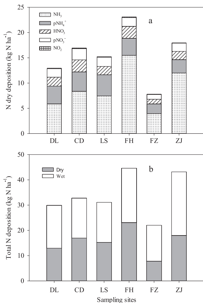
Figure 3. Atmospheric N dry deposition (a) and total deposition (b) rates at the sampling sites.
