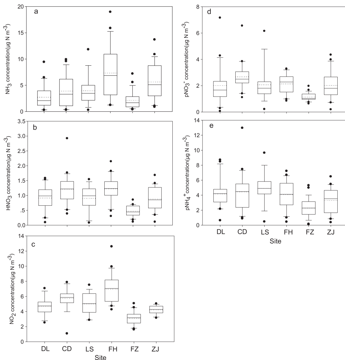
Figure 2. Atmospheric concentrations of reactive N ((a) \text{NH}_3 , (b) \text{HNO}_3 , (c) \text{NO}_2 , (d) \text{pNO}_3^- , (e) \text{pNH}_4^+ ) at six sites during sampling periods. Solid line represents median values and dotted line represents average values.
