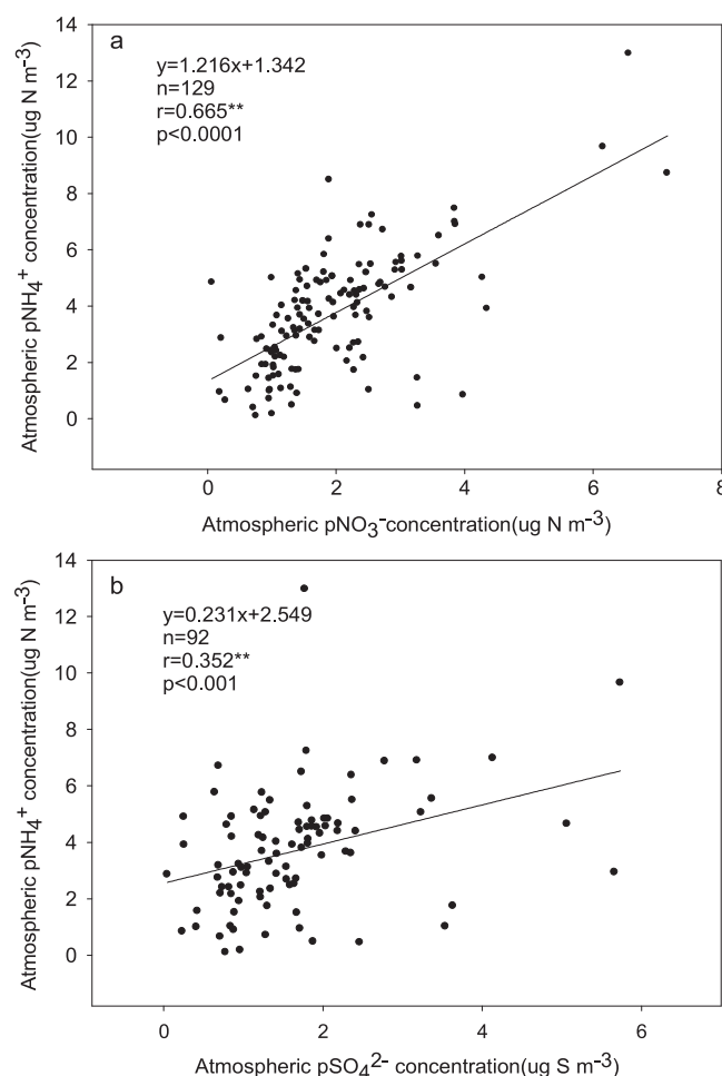
Figure 4. Relationship between atmospheric \text{pNH}_4^+ and \text{pNO}_3^- (a) and/or \text{pSO}_4^{2-} (b).
