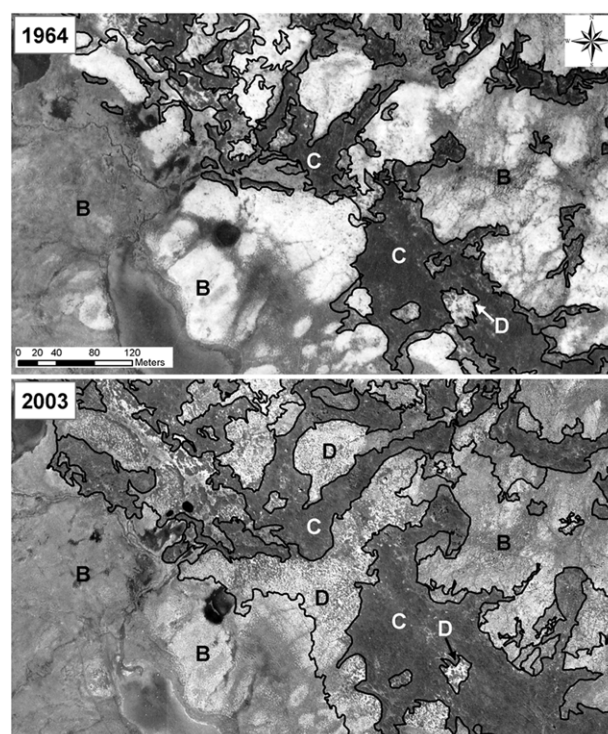
Figure 3. Portions of the 1964 and 2003 orthophotos showing examples of erect shrub cover for the three cover types: <10\% (B for barren), discontinuous (D) and continuous (C). Darker shade of erect shrubs is easily seen in discontinuous and continuous areas, but distinct texture is most evident in the continuous cover polygons. Dark grey tones in the <10\% erect shrub cover (barren) areas correspond to wet vegetation (fens) with dense mosses, herbs and prostrate shrub cover and some exposed gravel and boulders on better drained microsites. Top panel reprinted with permission from Natural Resources Canada 2012, courtesy of the National Air Photo Library (A18324-19 (1964-08-06)). Bottom panel reproduced with permission from Géoboutique Québec, Ministère des Ressources naturelles et de la Faune (24I12-1602 and 1702 (2003-07-23); © Government of Québec).
