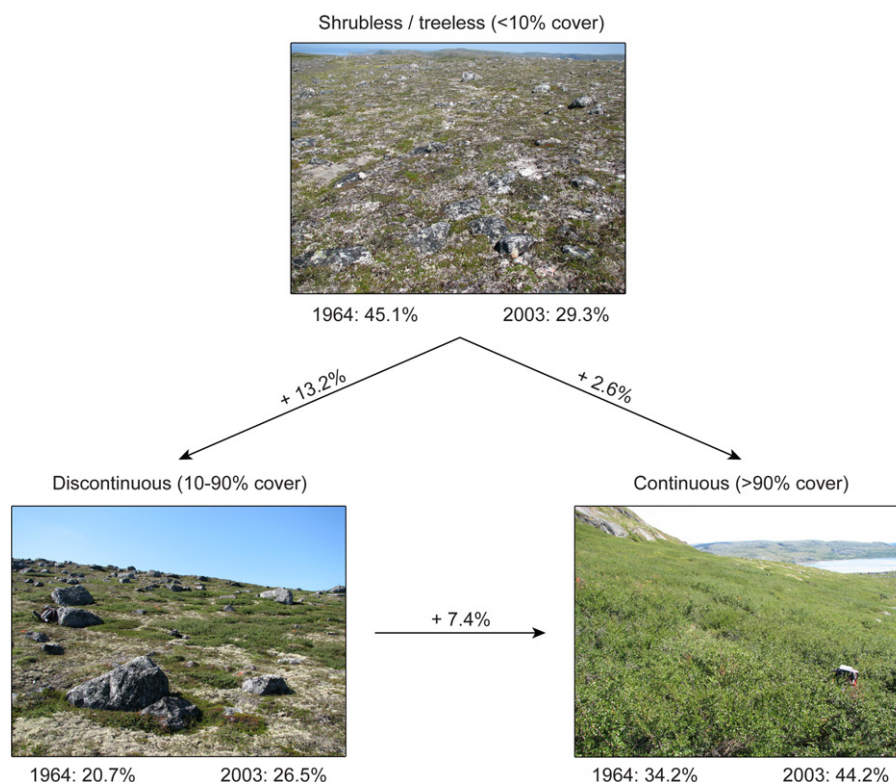
Figure 4. Changes in erect woody vegetation cover in the vicinity of Kangiqsualujjuaq (Nunavik, Québec) from 1964 to 2003 detected through comparative analysis of past and recent aerial vertical orthophotos. All values are in per cent and represent proportions of studied area. Arrows show direction of change from one vegetation cover type to another, accompanied by amount of change indicated above.
