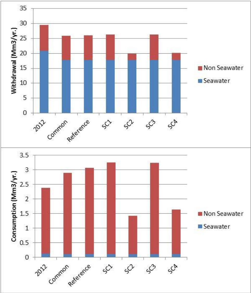
Figure 2. Thermoelectric water use by the WECC region in 2012, the 2022 Common Case and for each five scenario study cases. The top graph shows water withdrawals, while the bottom provides water consumption. Values include the U.S. region only.
