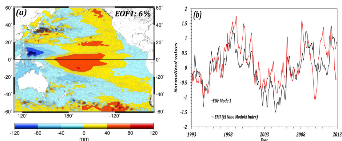
Figure 3. (a) Spatial pattern and (b) its corresponding time curve of the first EOF mode of Altimetry-IPO residual signal over 1993–2013. The EMI index is represented as the red curve.
