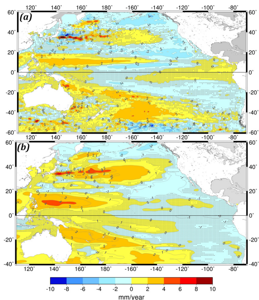
Figure 2. (a) Altimetry and (b) 2D reconstruction-based Pacific Ocean sea level spatial trend pattern without IPO over 1993–2013 (uniform global mean has been removed from both before performing the regression. In the case of 2D reconstruction, regression was performed over 1960–2013 and the result is plotted over 1993–2013). Stippling indicates regions of non-significant trend ( p -value > 0.05 ).
