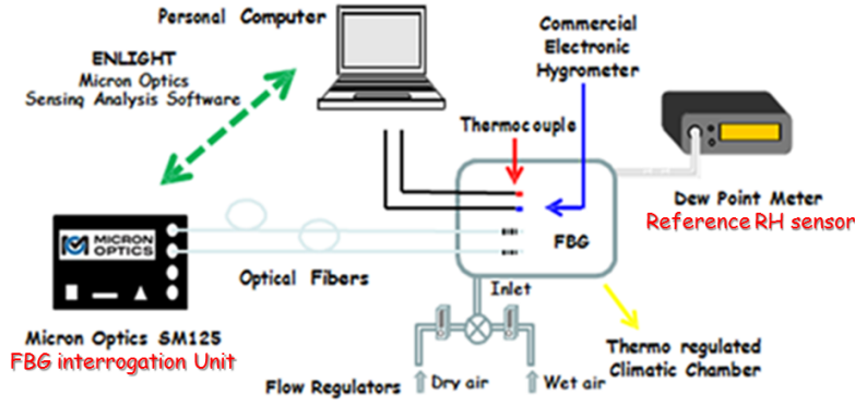
Figure 3. Experimental Set-Up.
