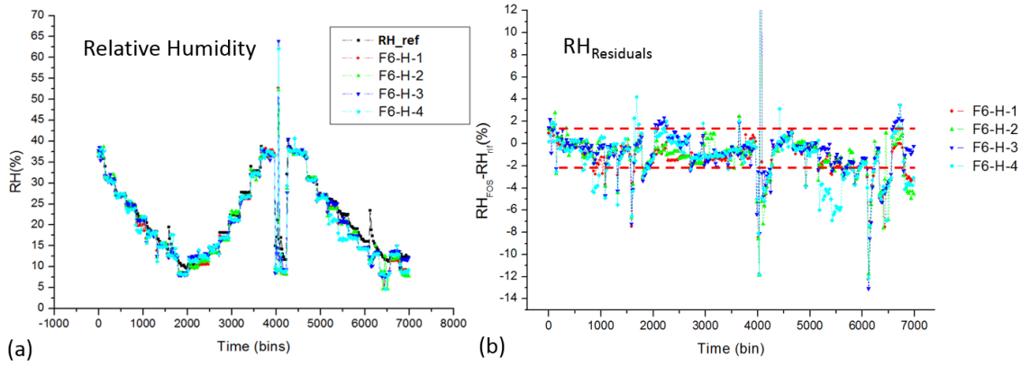
Figure 7. RH measured by a sample of four FOS Thermo-Hygrometer (a) with residuals (b).
