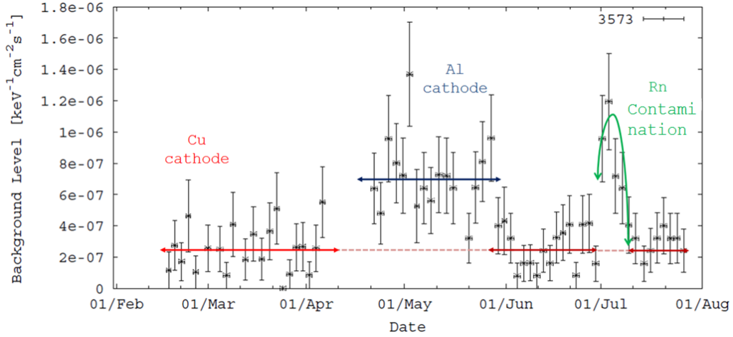
Figure 12. Ultra-low background period (2011) twice interrupted because of the replacement of the cathode's material and radon contamination.
