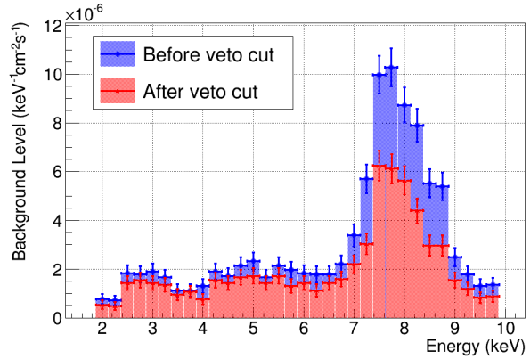
Figure 16. Left: current installation of a cosmic muons veto in the sunset Micromegas setup. Right: sunset Micromegas background accumulated during the summer 2012 data taking campaign by detector 1, before and after applying the cosmic rays veto.
