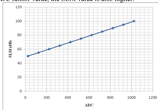
Figure 6. Noise Level Calibration Graph.
