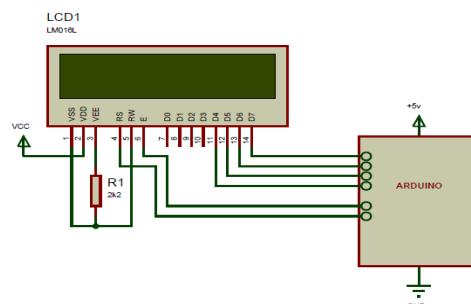
Figure 3. Series LCD which is connected with the arduino
