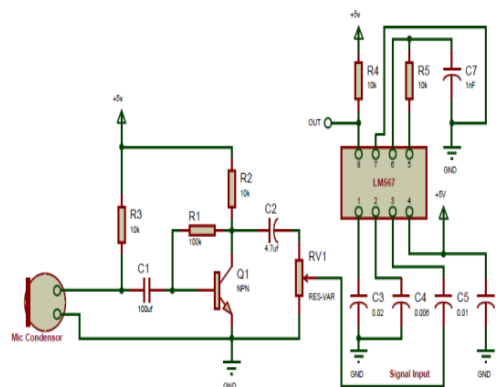
Figure 2. Noise detector sensor circuit.
