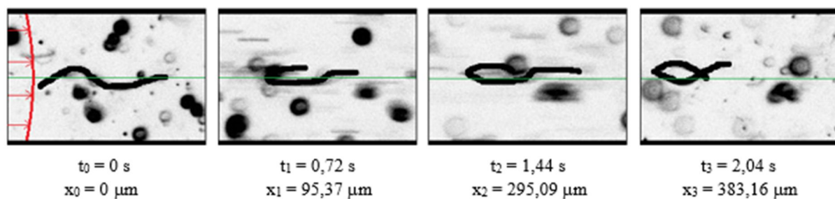
Figure 3. Sequence of images for a single flexible nanoflament conveyed by Poiseuille flow (no. 6 in Table 1), green line represents the center of the channel, t – time stamp, x – distance traveled from the channel entry (picture frame moves with the object), image height 77 \mu m ; negative of the images shown.
